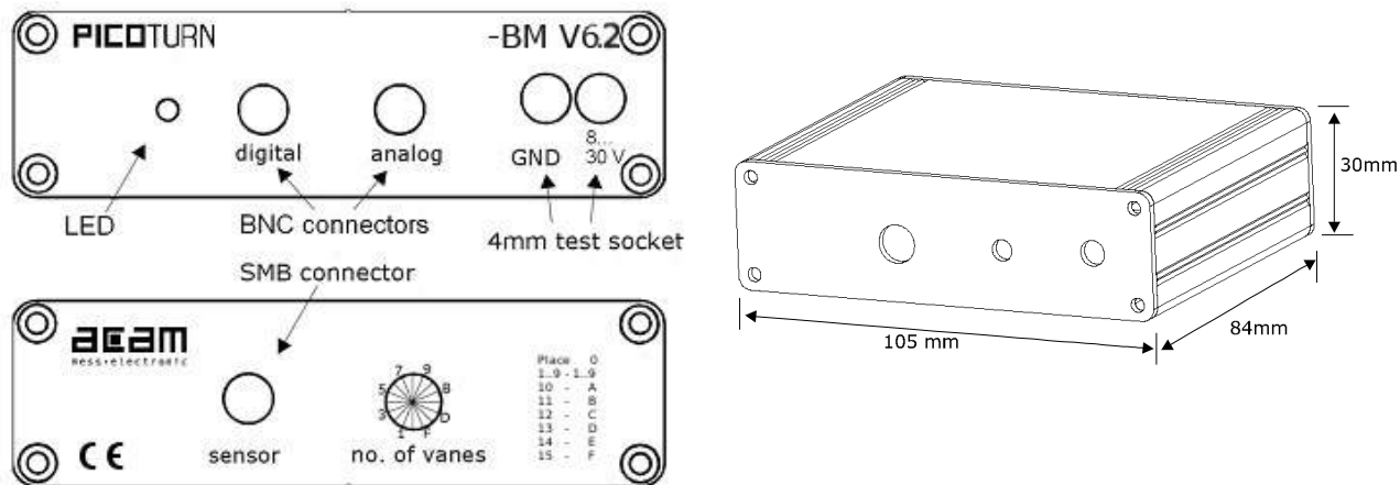
Figure 4: PTBM Outline
