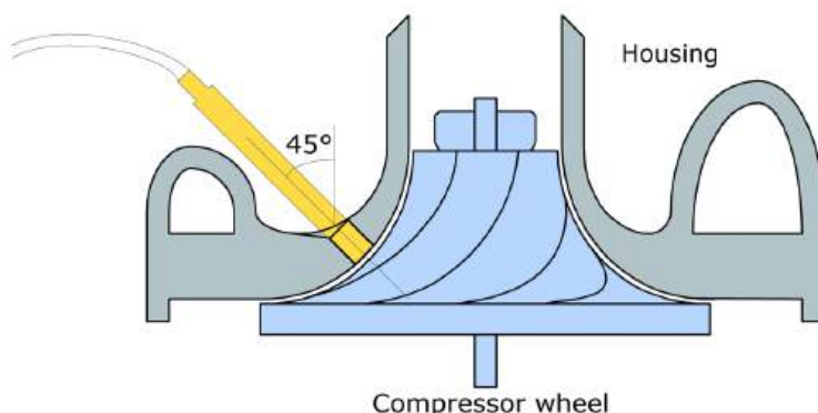
Figure 5: Sensor Application
