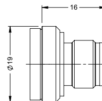
Connettore M12x1 4-PIN temperature standard (TB)
