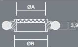
ISO-KF centering ring with sinter filter, stainless steel / Viton® / sinter bronze
