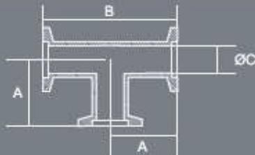
ISO-KF T piece, Aluminum
