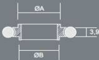
ISO-KF adaptive centering ring, stainless steel / Viton®
