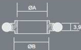
ISO-KF centering ring, stainless steel / Viton®
